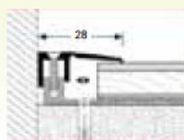
Type 287 | L Profile 7-16mm (without lifter).
