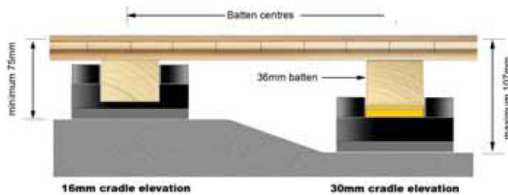
Section showing typical floor depths using the C1 Cradle
